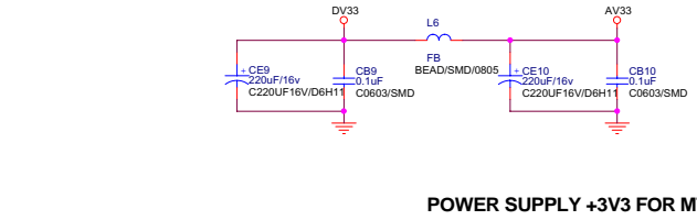
POWER SUPPLY +3V3 FOR MT5351 (ANALOG)
