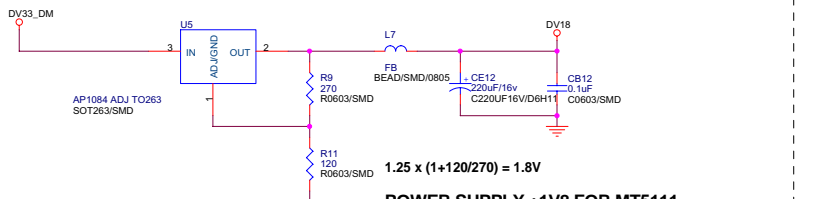
1.25 x (1+120/270) = 1.8V POWER SUPPLY +1V8 FOR MT5111
