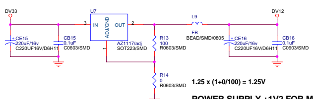
1.25 x (1+0/100) = 1.25V POWER SUPPLY +1V2 FOR MT5351
