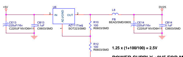
1.25 x (1+100/100) = 2.5V POWER SUPPLY +2V5 FOR MT5351 AND DDR
